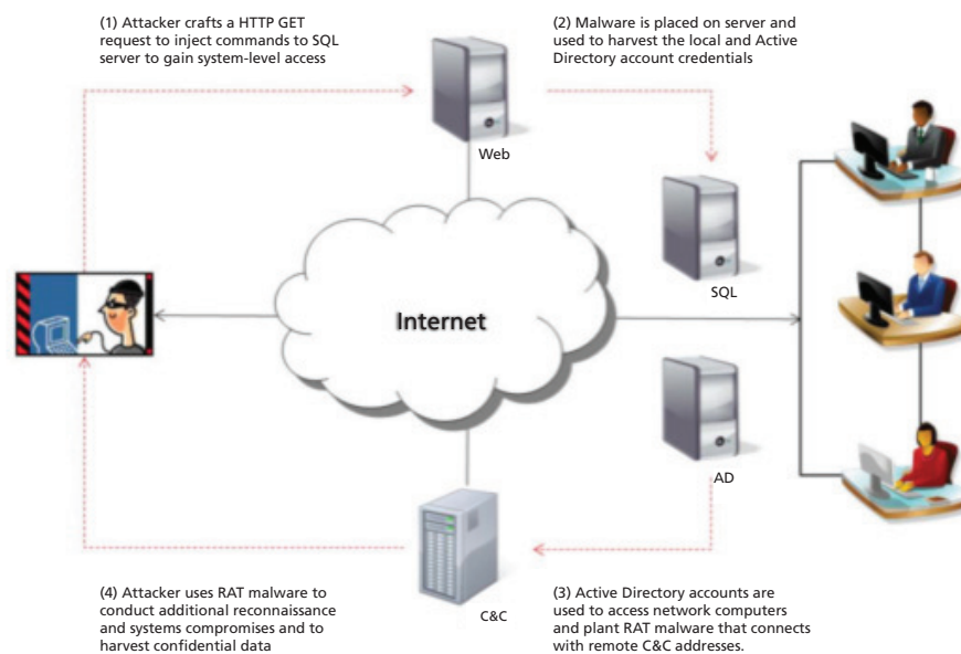
Figure 2. SQL-injection attacks.
